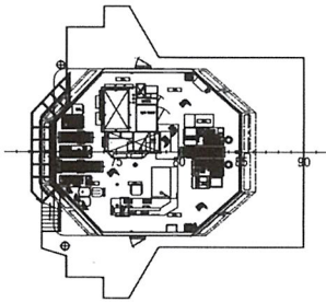
C - DECK
