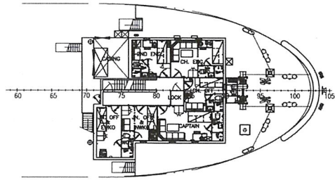
B - DECK
