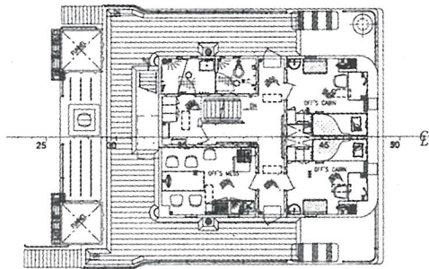
UPPER DECK
