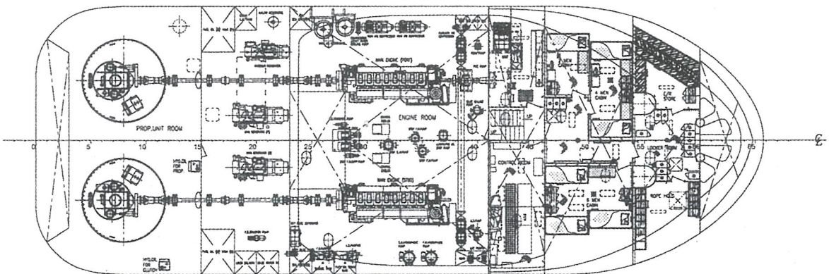
UNDER DECK
