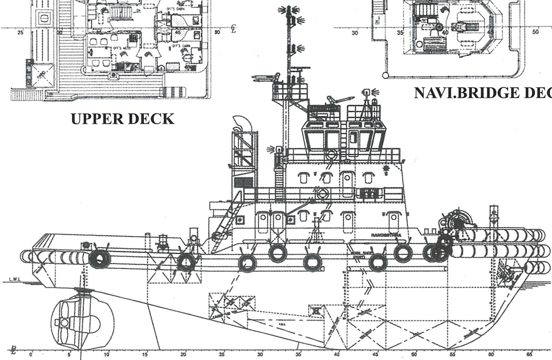
PROFILE
