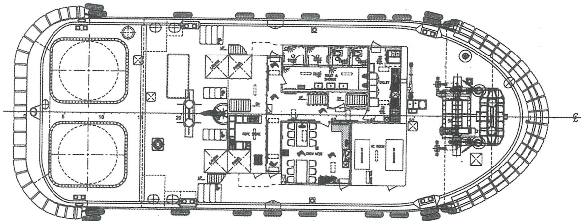
MAIN DECK
