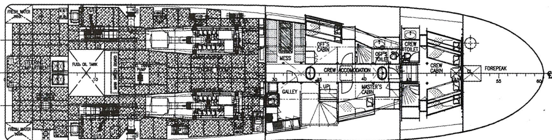
HOLD PLAN
