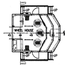
WHEELHOUSE PLAN
