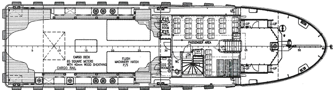
DECK PLAN
